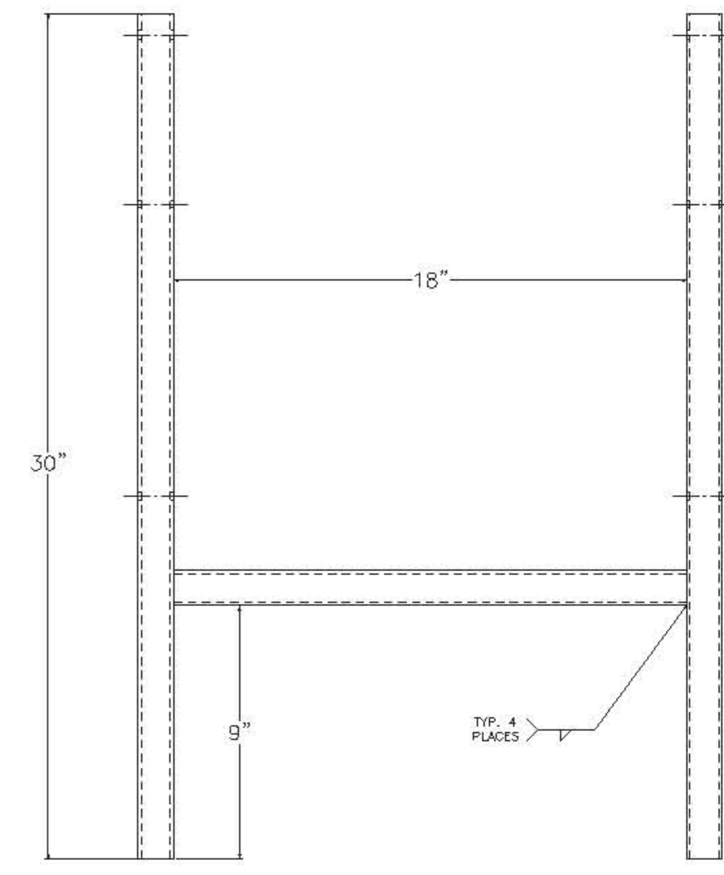
TYPICAL LEG ASSEMBLY
